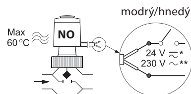
Obr. 3 TWA-Z NO a AB-QM
