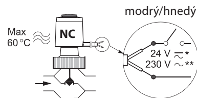
Obr. 4 TWA-Z NC a AB-QM
